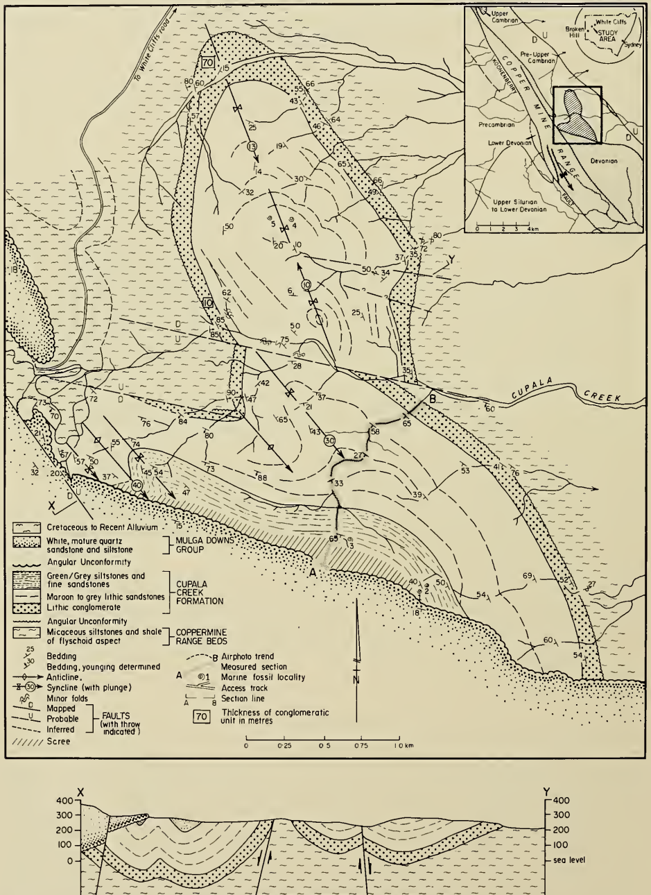
Fig. 1. Geological map and cross section of the Cupala Creek Formation.
